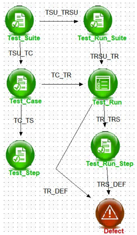
Figure 5-1. Test Management Class Definition
