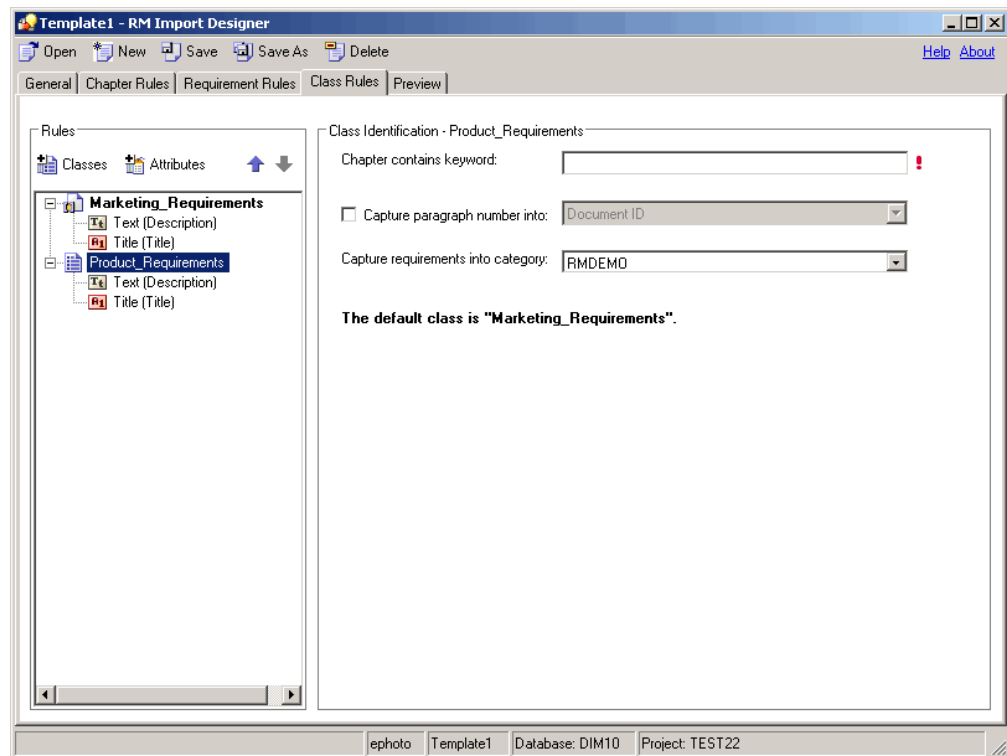
Figure 5-10. Class Rules Tab—Non-Default Class
