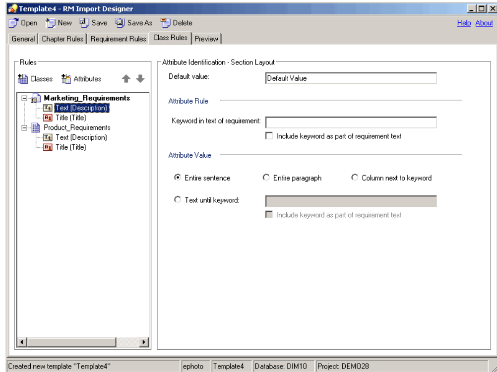
Figure 5-15. Class Rules Tab—Section or Keyword Option—Text or Numeric Attributes
