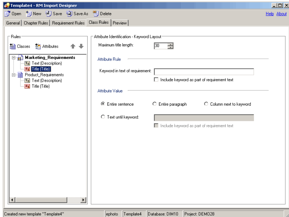
Figure 5-13. Class Rules Tab—Section or Keyword Option—Alphanumeric Attributes
