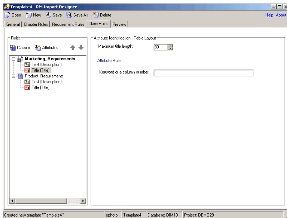
Figure 5-14. Class Rules Tab—Table Option—Alphanumeric Attributes
