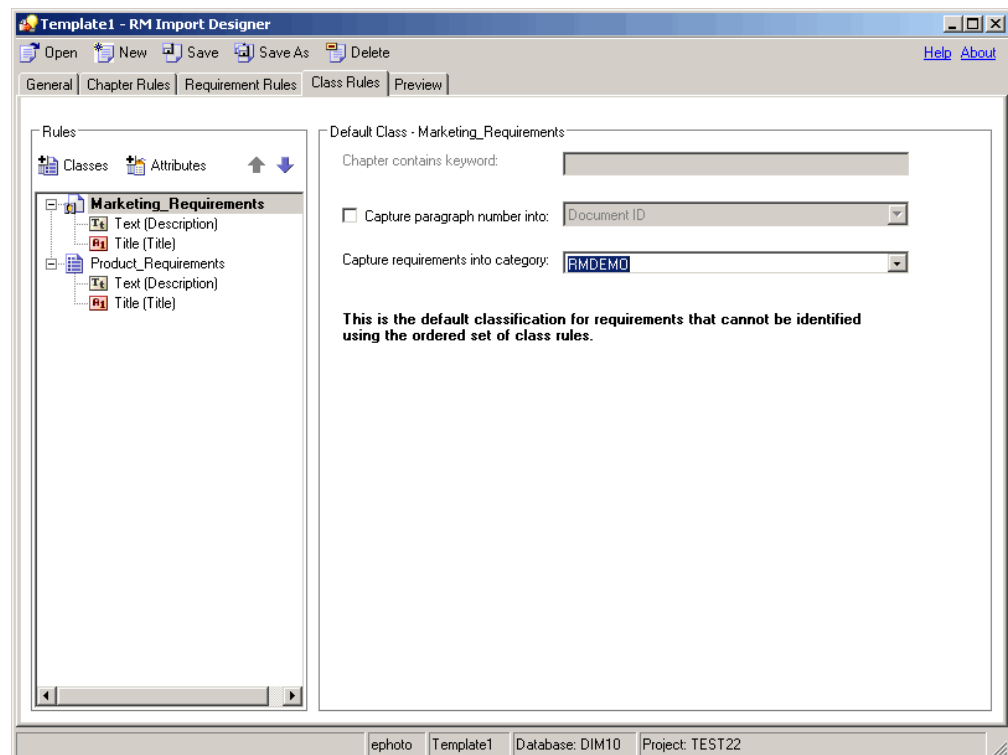
Figure 5-9. Class Rules Tab—Default Class
