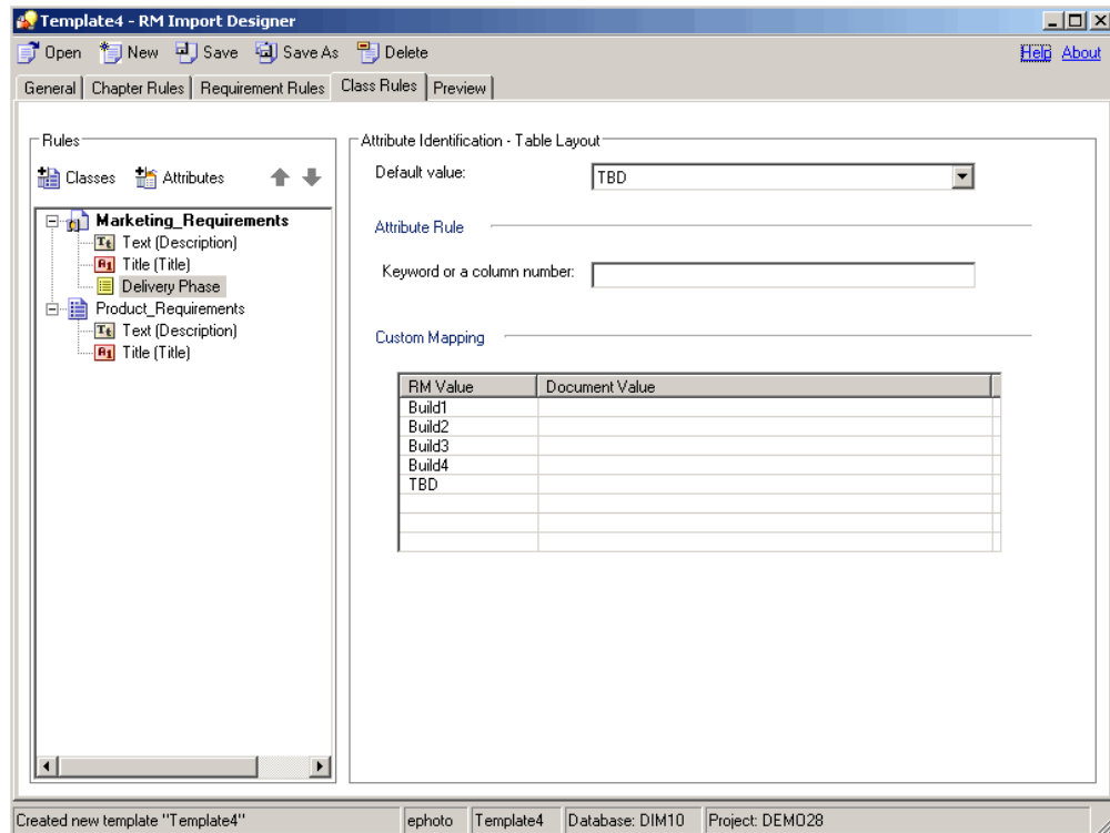
Figure 5-18. Class Rules Tab—Table Layout—List Attributes
