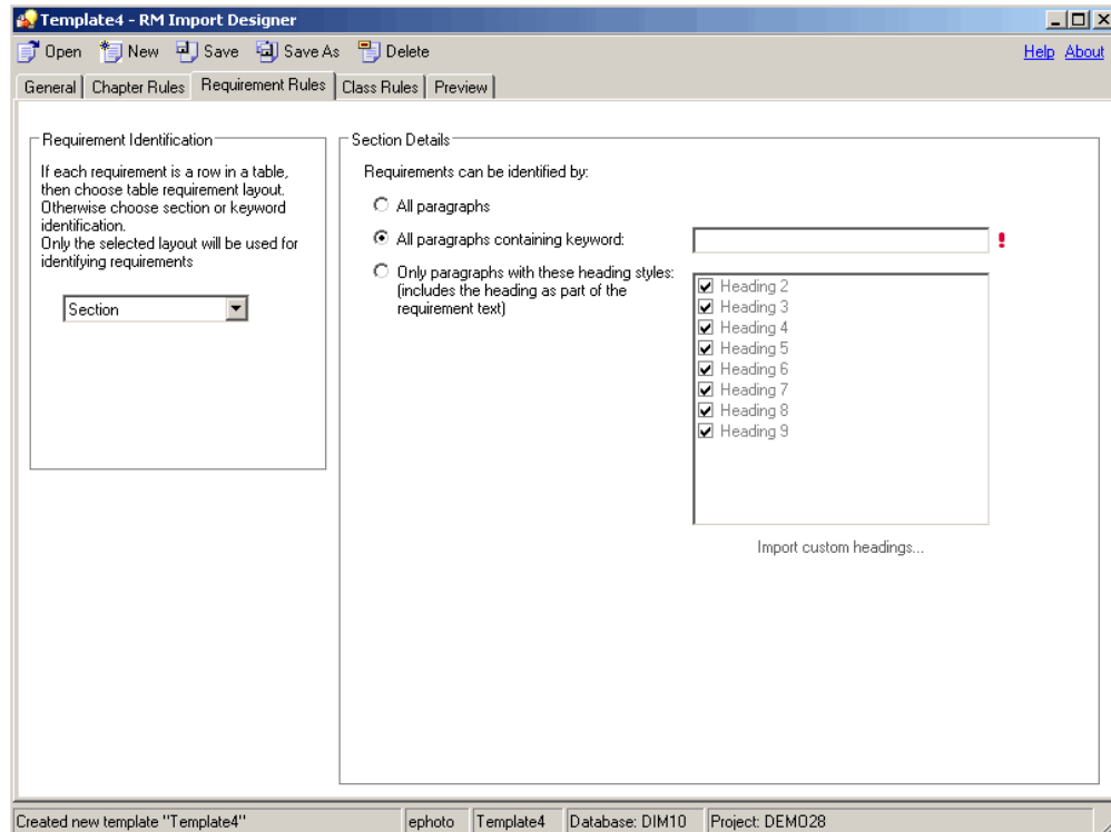
Figure 5-7. Requirement Tab—Section Option
