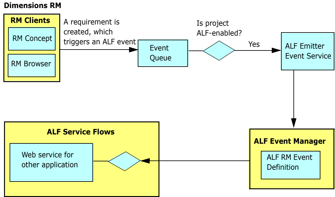
Figure 6-2. Emitting an Event from Dimensions RM
