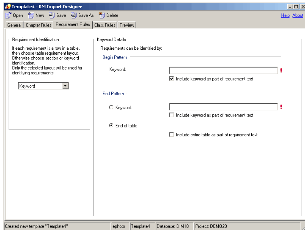
Figure 5-8. Requirement Tab—Keyword Option
