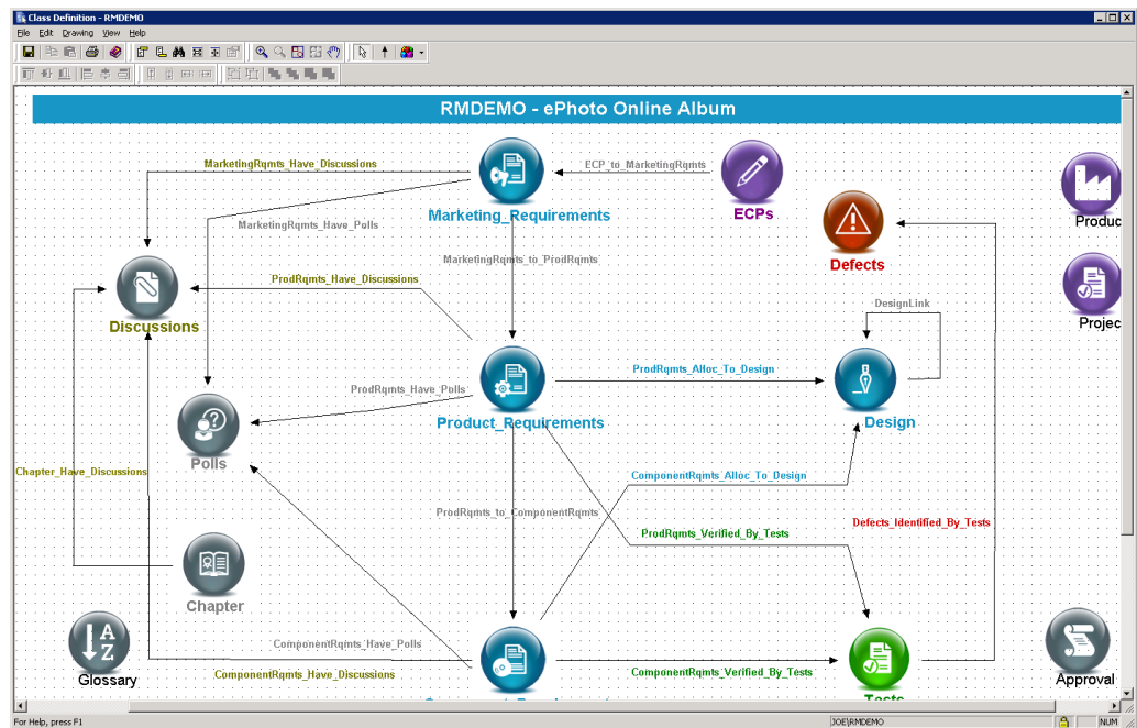
Figure 1-4. Class Definition
