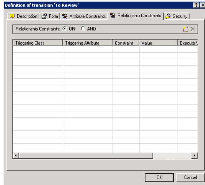
Figure 9-30. Relationship Constraint Settings dialog
