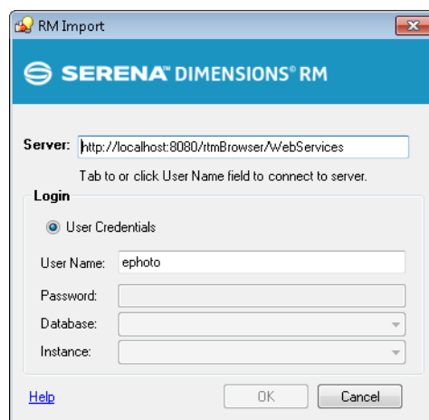
Figure 12-1. Login Dialog
