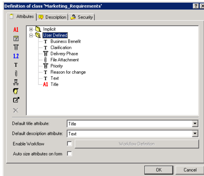
Figure 9-17. Class Definition
