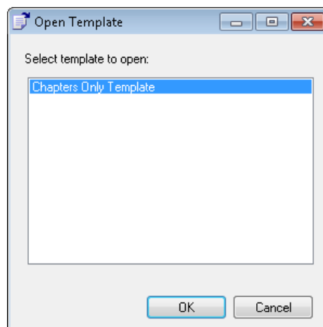
Figure 12-2. Open Template
