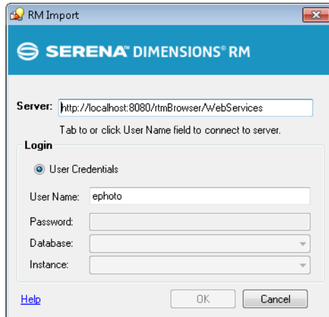
Figure 11-1. Login Dialog
