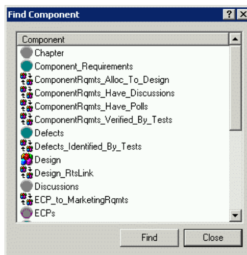
Figure 9-4. Find Component
