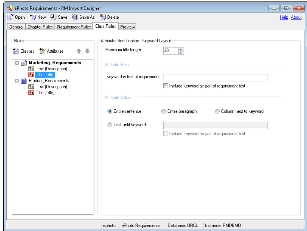
Figure 12-13. Class Rules Tab—Section or Keyword Option—Alphanumeric Attributes
