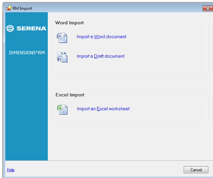
Figure 1-1. RM Import
