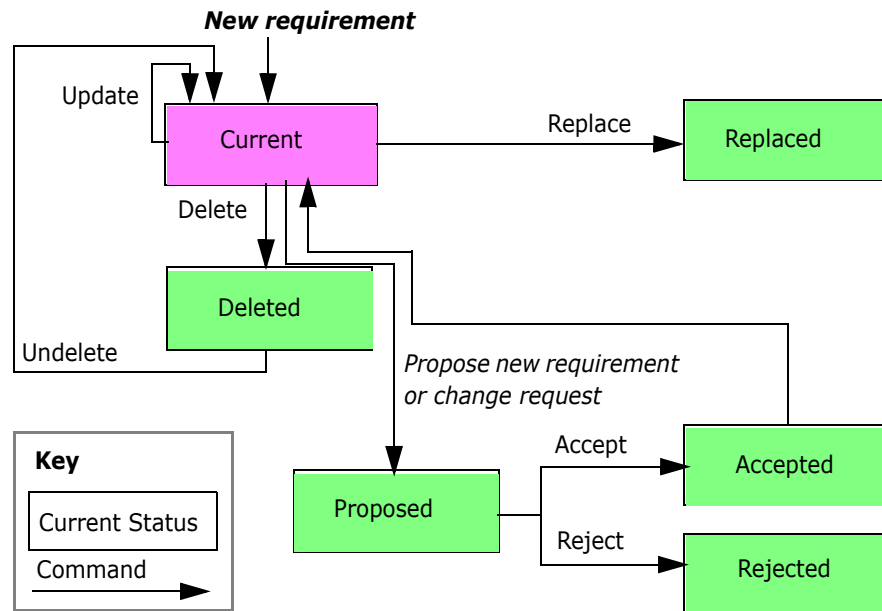
Figure 1-6. Object Lifecycle
