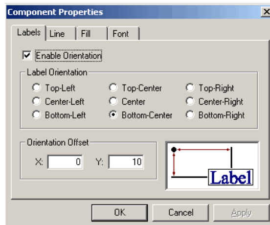
Figure 9-24. Component Properties
