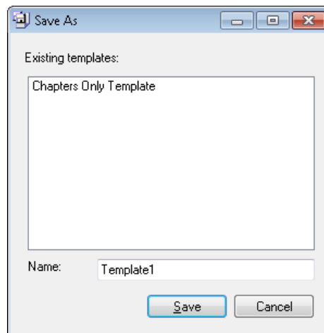
Figure 12-3. Save As
