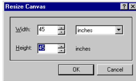
Figure 9-3. Resize Canvas
