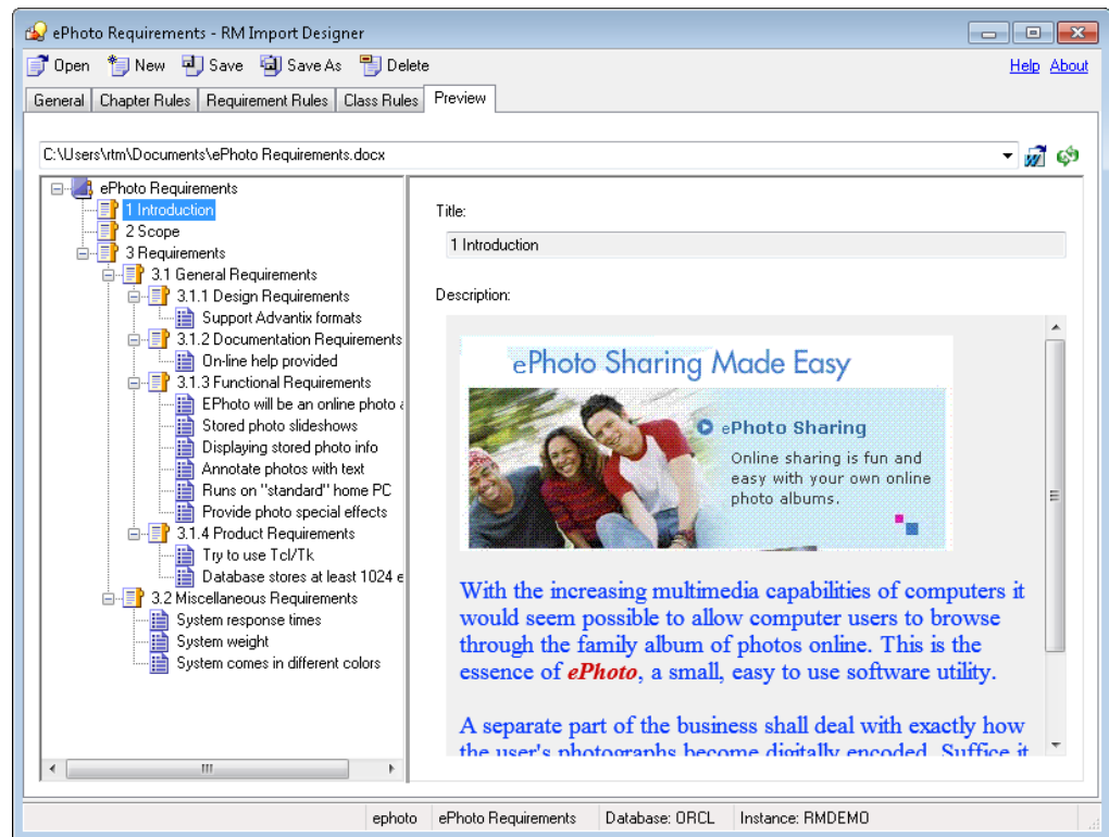
Figure 12-20. Preview Tab
