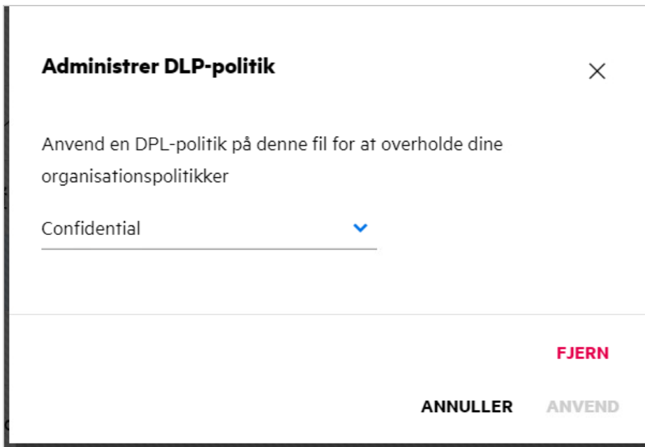
Figure 58 Administrer DLP-politik
