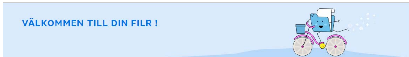
Figure 1 Sidan Start
