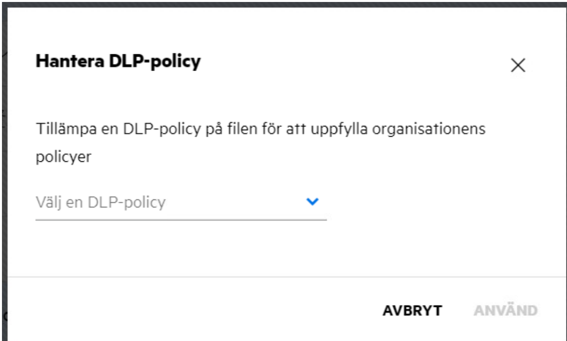
Figure 55 Hantera DLP-princip
