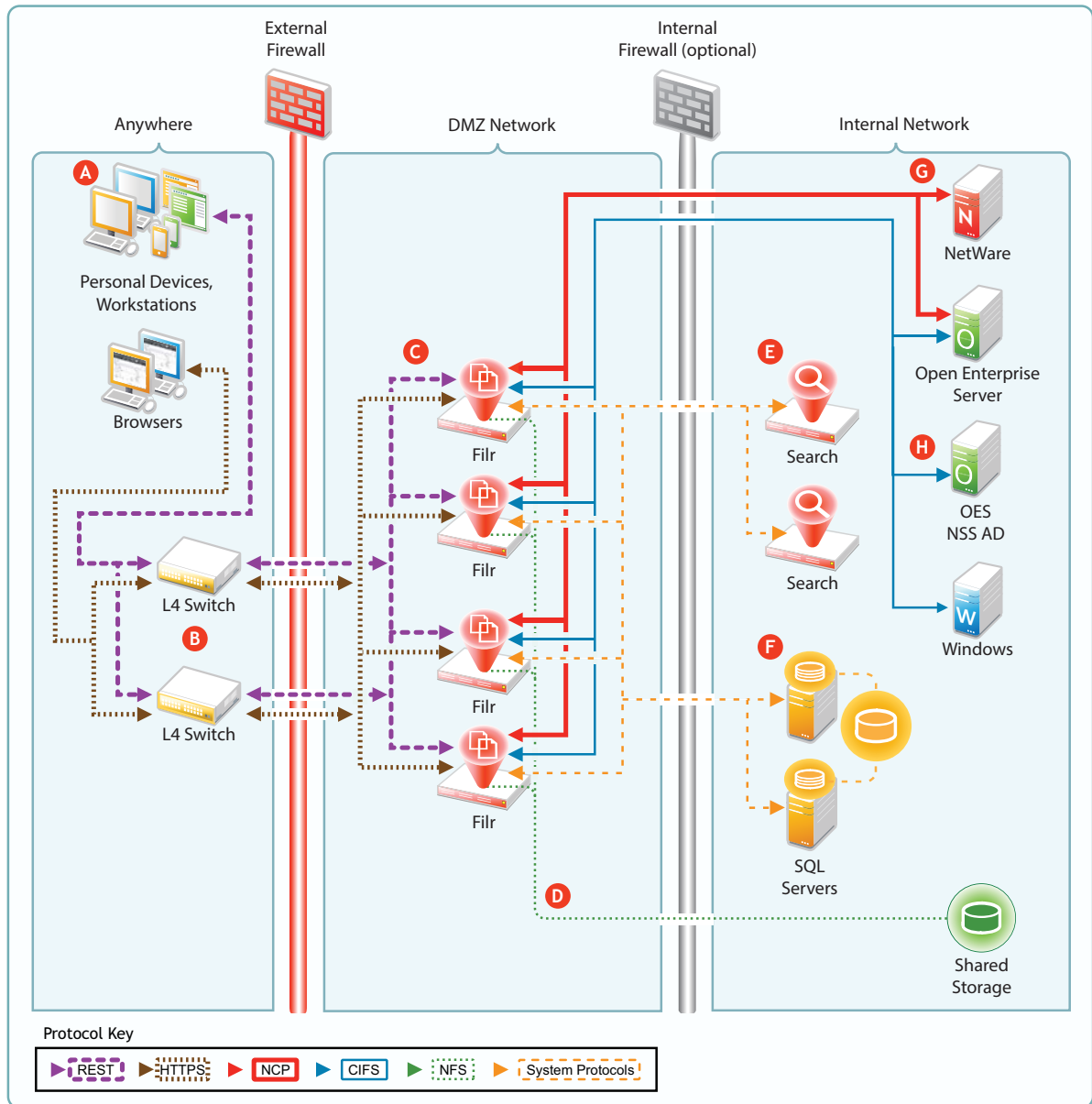
Figure 2-13 Example of a Large Filr Deployment
