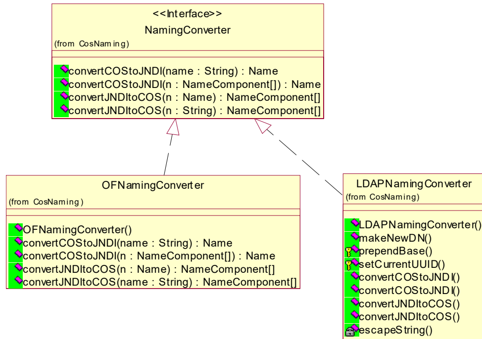
Figure 6 OFNamingConverter Interface
