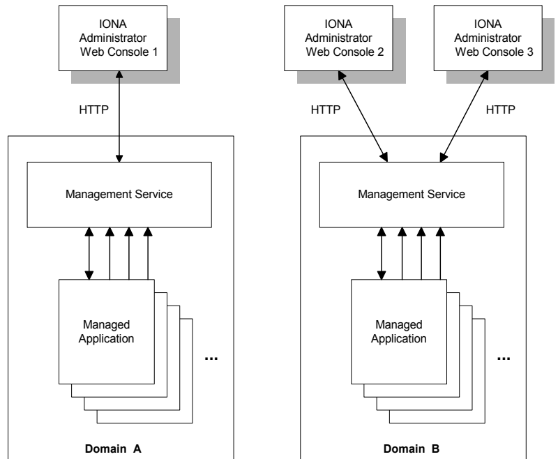
Figure 3: IONA Administrator Architecture
