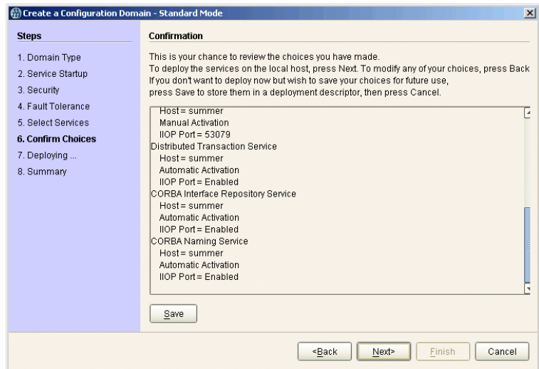
Figure 12: Confirmation Screen
