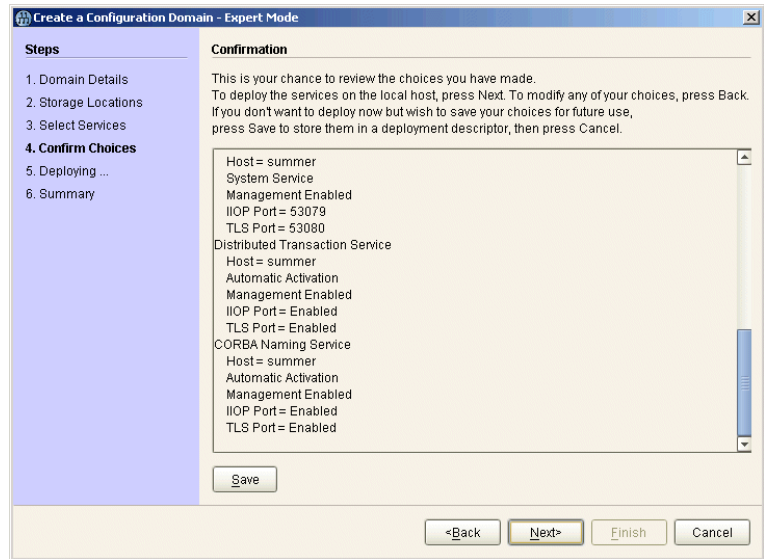
Figure 27: Confirmation Screen
