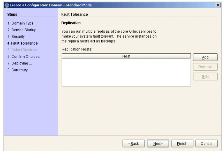
Figure 9: Replica Configuration
