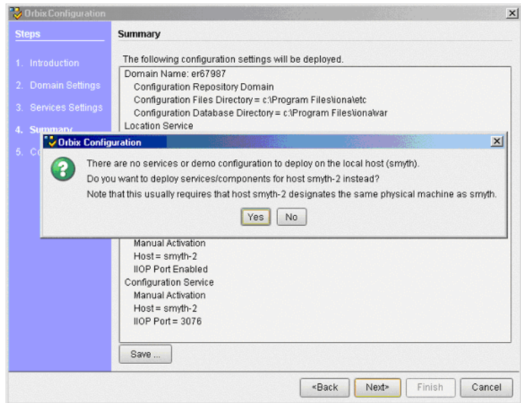
Figure 30: Multi-homed Message
