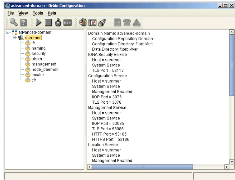
Figure 18: Loaded Domain
