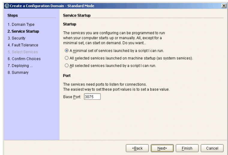
Figure 7: Startup Mode and Base Port
