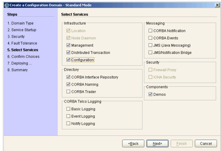
Figure 11: Selecting Services to Deploy
