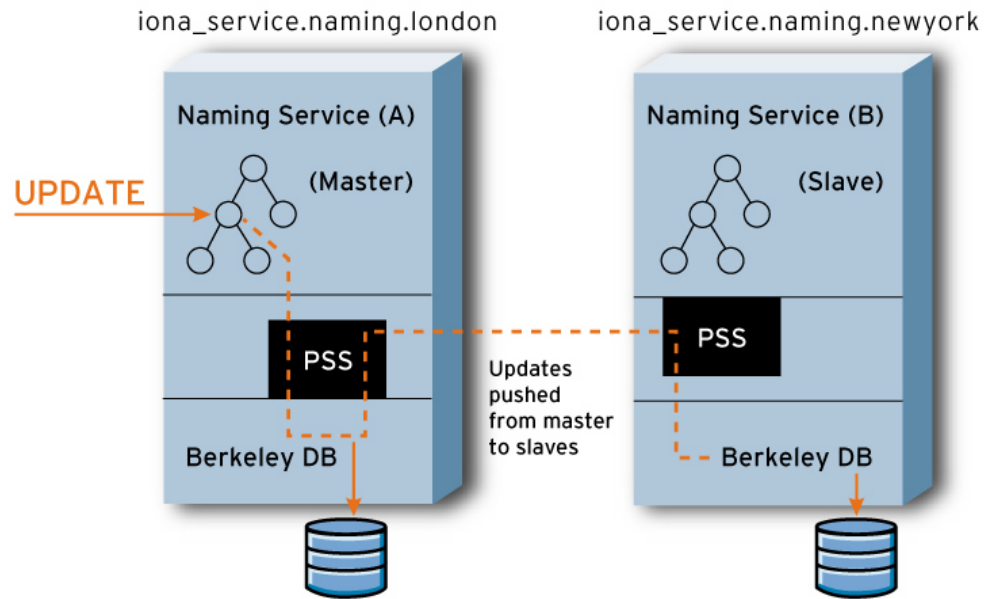
Figure 7: Orbix Replication
