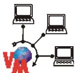
Desktop client
