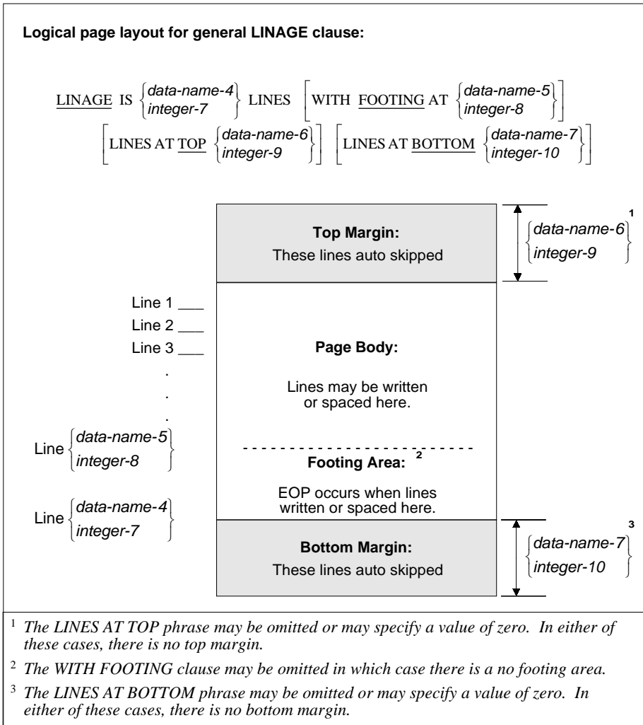
Figure 4-1: General LINAGE Clause
