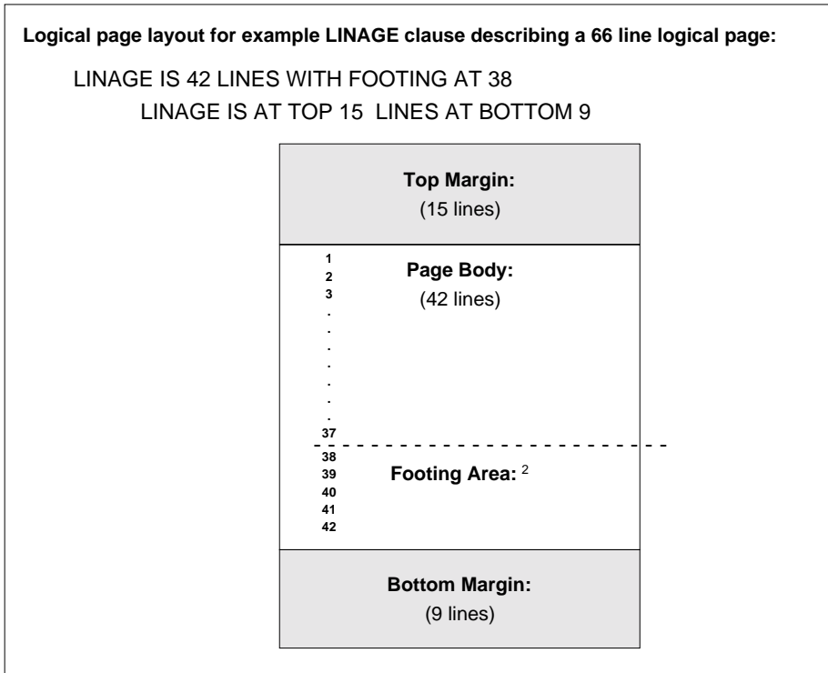
Figure 4-2: Example LINAGE Clause
