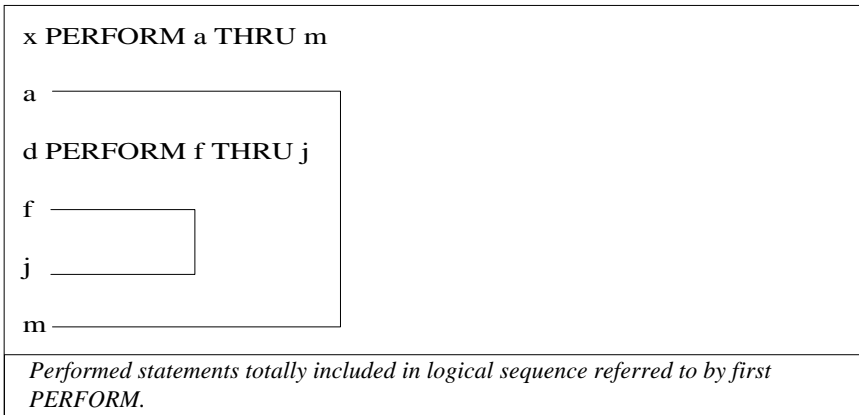
Figure 6-5: PERFORM Statement Examples
