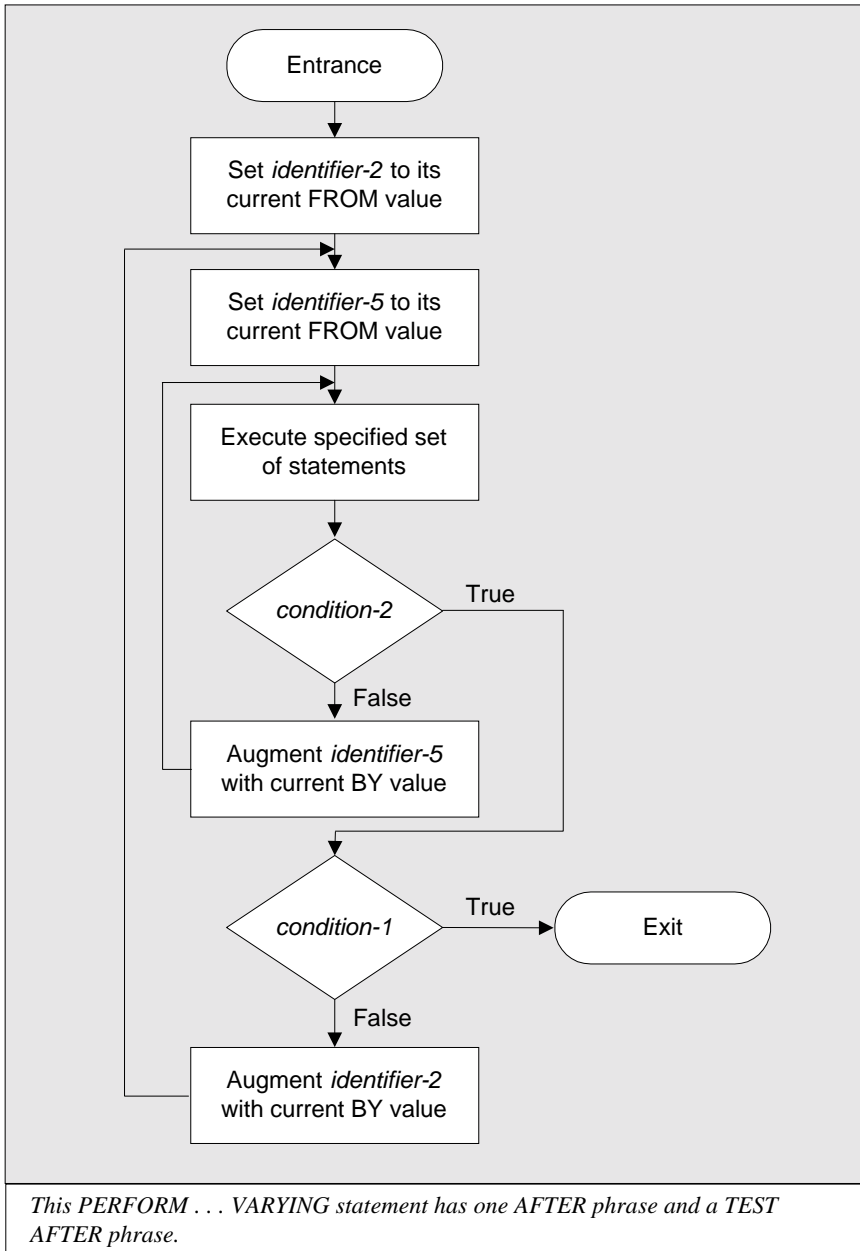
Figure 6-4: PERFORM . . . VARYING Statement
