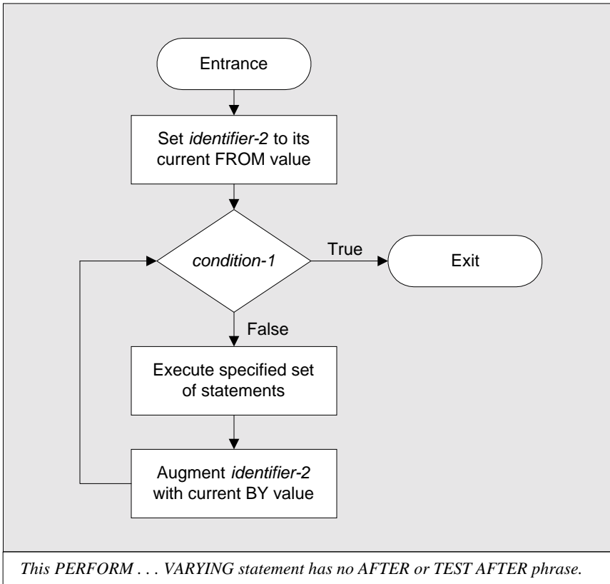
Figure 6-1: PERFORM . . . VARYING Statement
