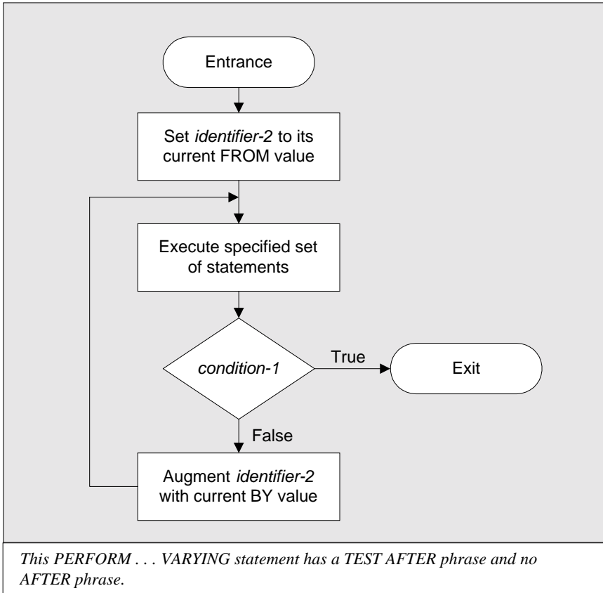
Figure 6-3: PERFORM . . . VARYING Statement
