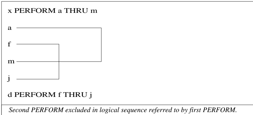
Figure 6-7: PERFORM Statement Examples
