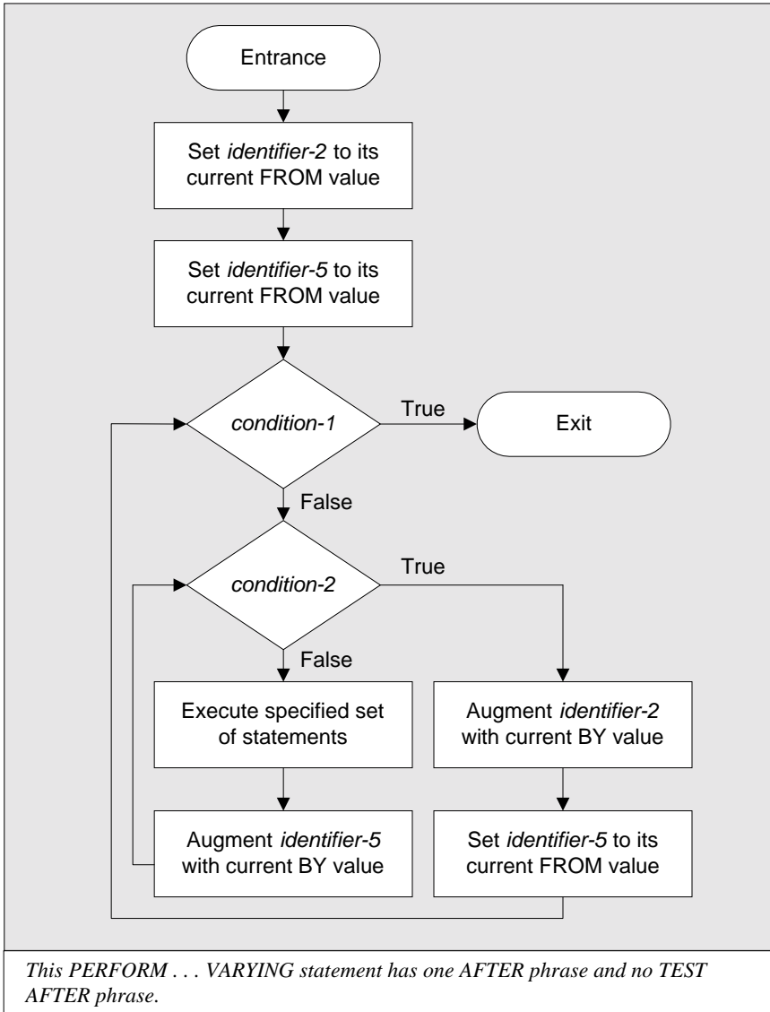
Figure 6-2: PERFORM . . . VARYING Statement
