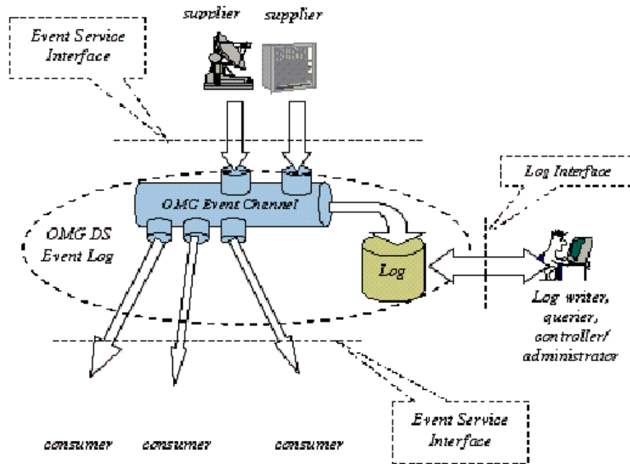
Figure 1 EventLog architecture
