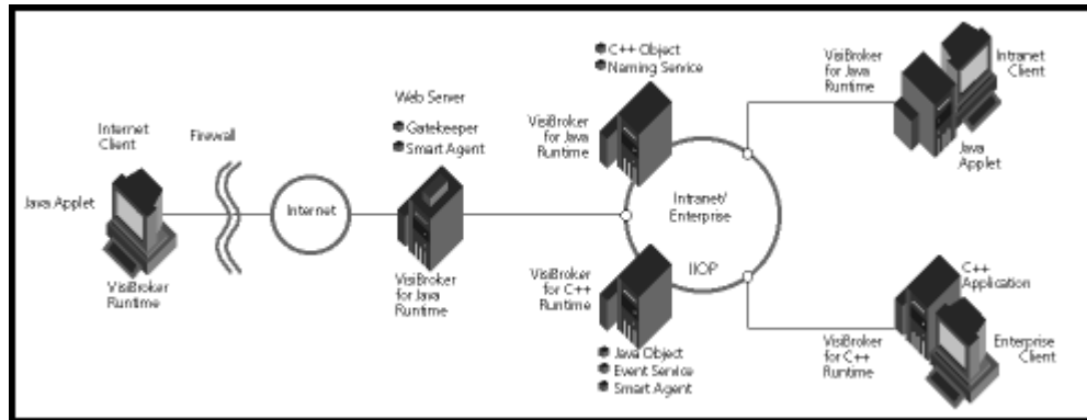
Figure 2 VisiBroker Architecture
