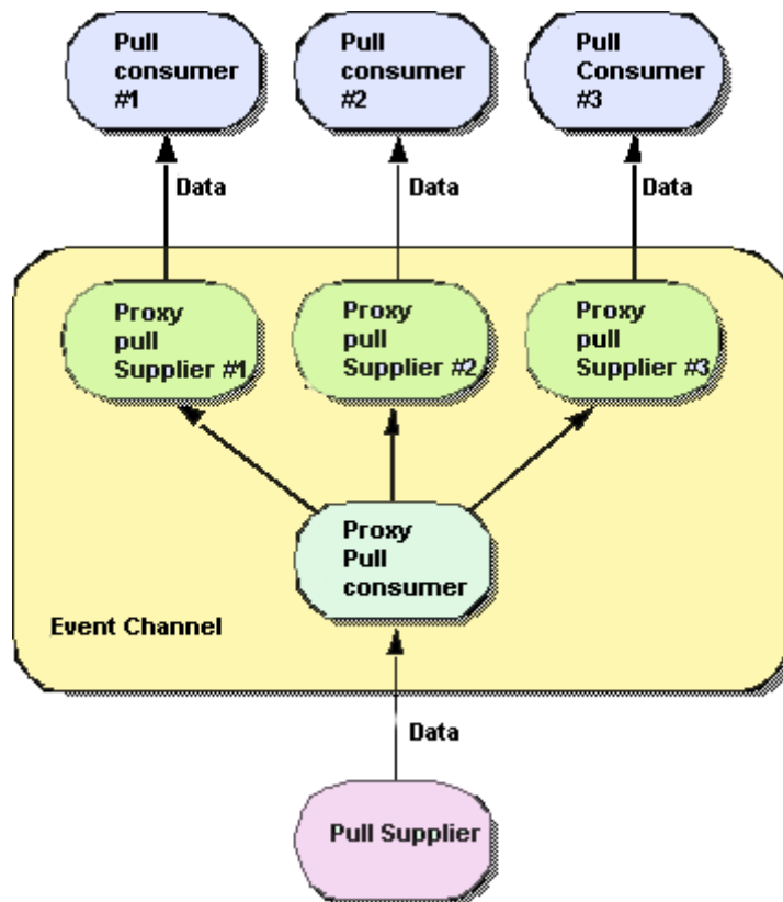
Figure 30 Pull model
